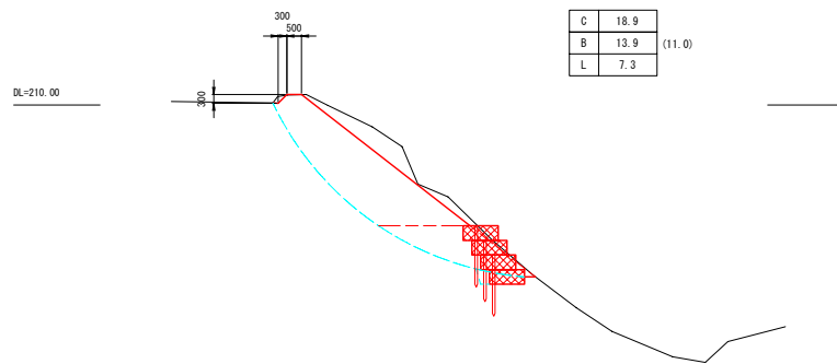
NO. 2 GH=210.00 FH=210.37
