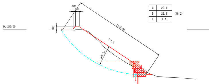
NO. 0 GH=210.41 FH=210.41
