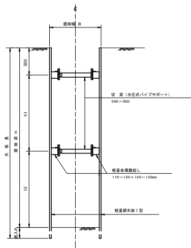
(切梁数2段)
